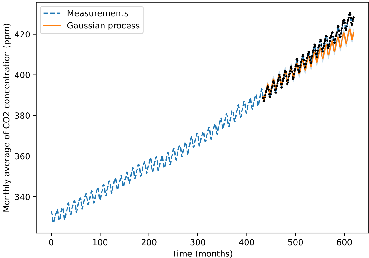
Monthly average of air samples measurements from the Mauna Loa Observ
